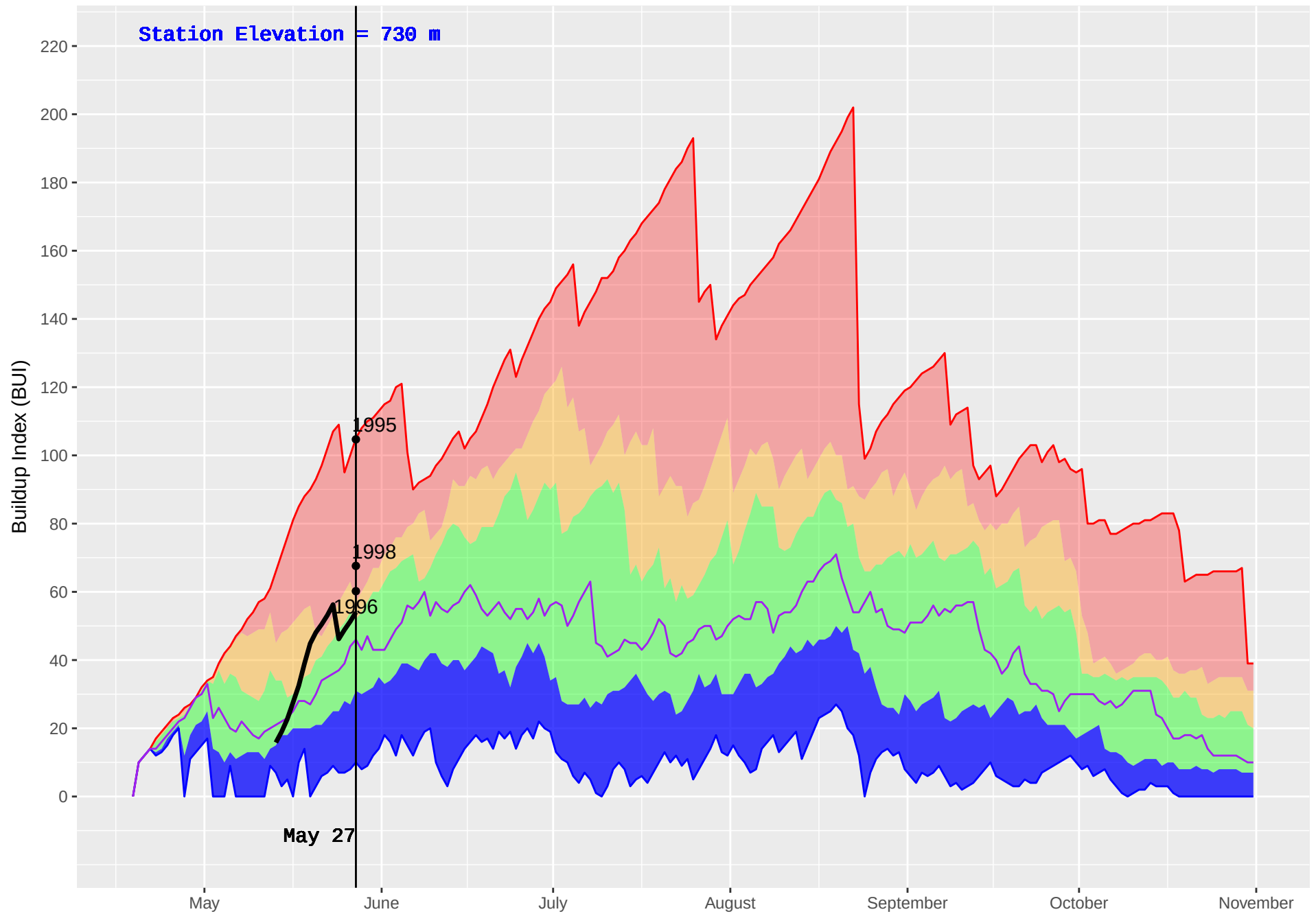
BOYA LAKE (445) : Historical (1985–2016) and Current (2018) Noon Buildup Index (BUI)
